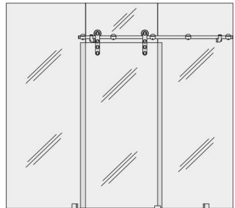
FLS404 glass mounted single slider with sidelite
