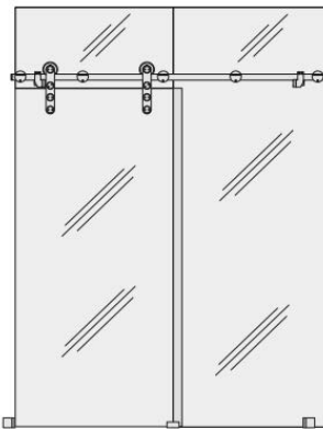
FLS403 glass mounted single slider
